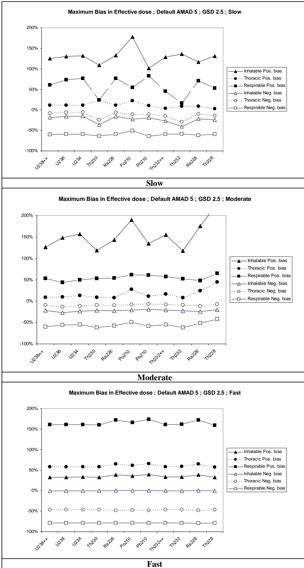
Figure 1: Maximum positive and negative bias (for a true AMAD between 1 and 20 \mu\text{m} ) between the estimated and true effective dose, for a default AMAD value of 5 \mu\text{m} and GSD 2.5 (Situation 4)
